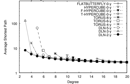
Figure 11. Average shortest path length vs. degree for random shortcut topologies generated using different base topologies ( N = 2^{10} vertices).
