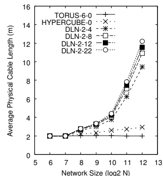
Figure 28. Average cable length vs. N for non-random topologies and random shortcut DLN with centralized switch layout.
