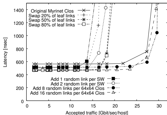
Figure 26. Latency vs. accepted traffic for random shortcut patterns on Myrinet Clos (80 switches, 256 hosts).
